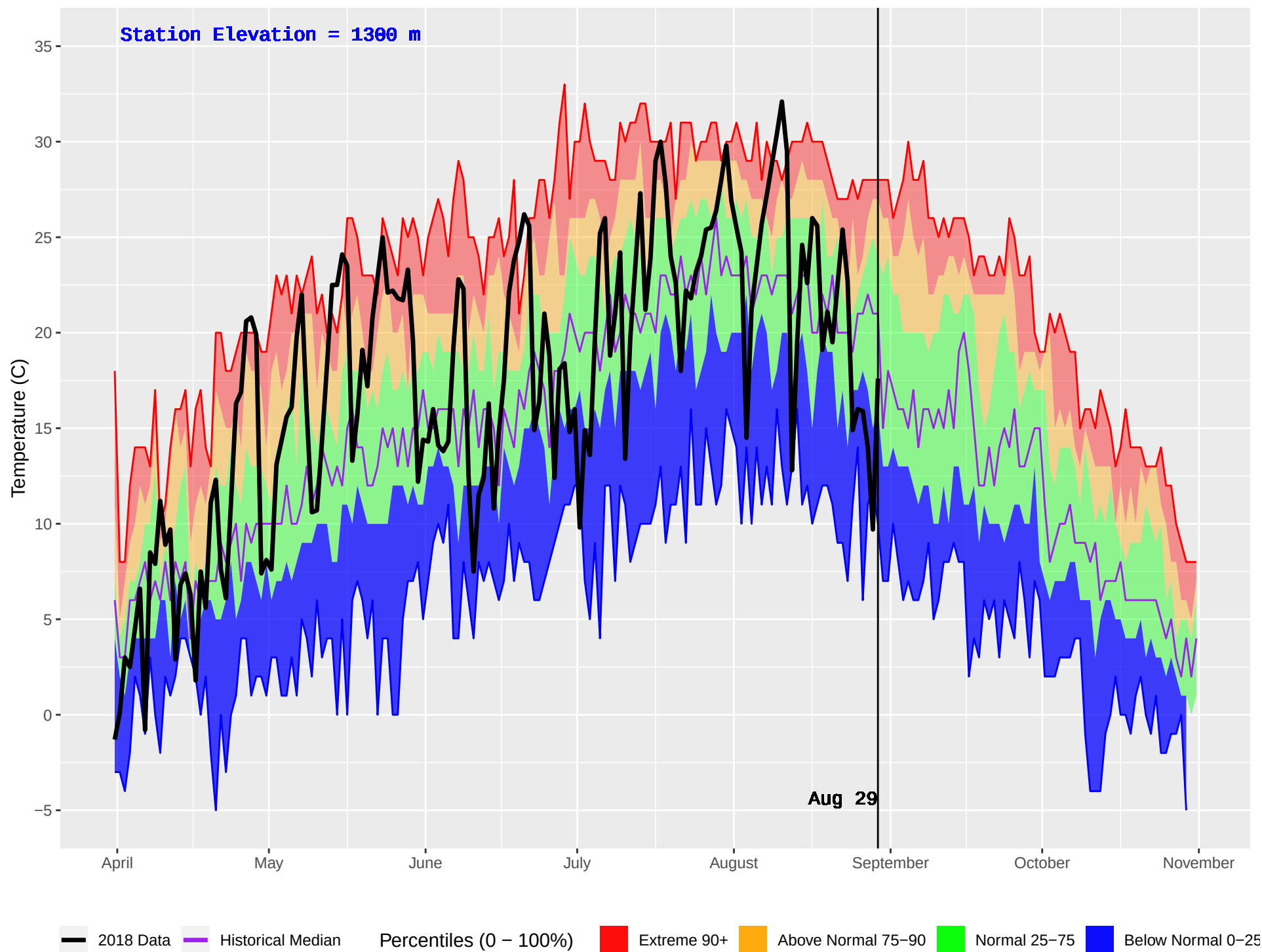
MARION (367) : Historical (1994–2016) and Current (2018) Daily Temperature
